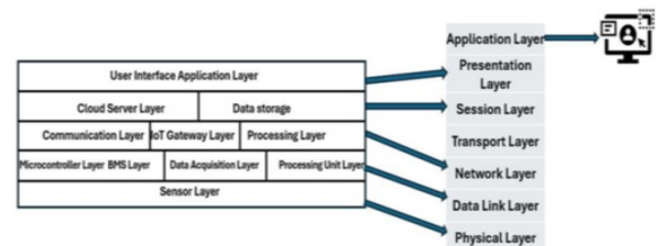
Fig. 2. Proposed 5 Layered IoT Architecture.
